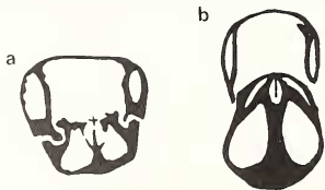
TEXT-FIG. 1. Serial sections showing internal structures of Ferganella turkestanica . Diagrams based on illustrations in Nikiforova (1937, pl. 7, figs. 15 and 16). Exact positions relative from posterior not known, but a is closer than b .
